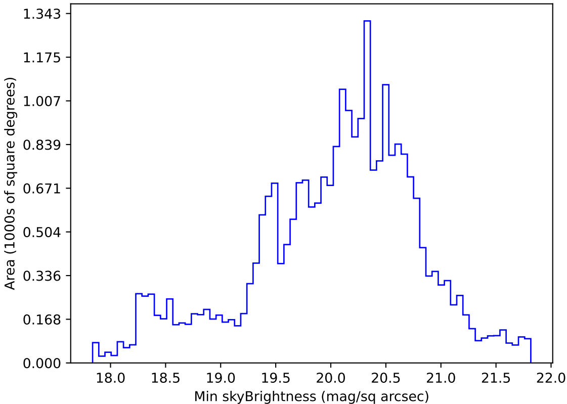
too_elab_r8_d2_ugrizy_v3.4_10yrs All sky g band: Min skyBrightness
