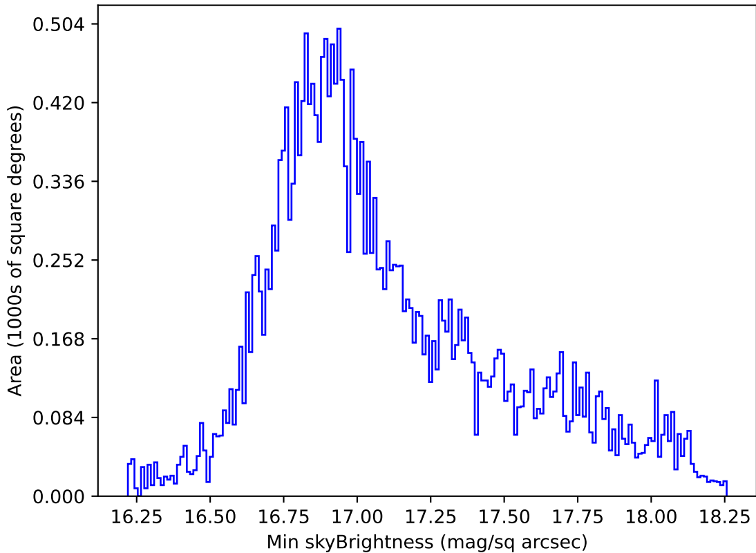
too_elab_r8_d2_ugrizy_v3.4_10yrs All sky all bands: Min skyBrightness
