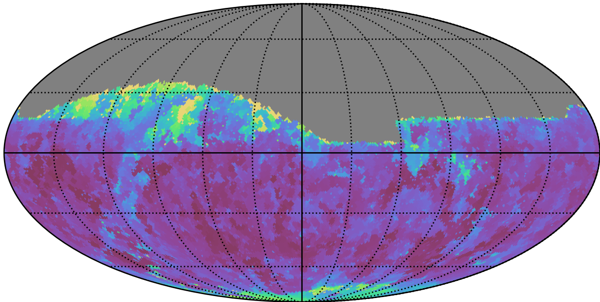
too_elab_r8_d2_ugrizy_v3.4_10yrs Yr 1 z band: Min seeingGeom
