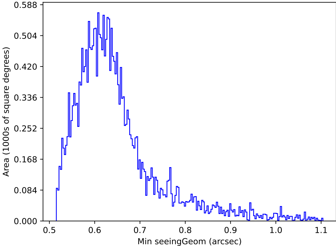
too_elab_r8_d2_ugrizy_v3.4_10yrs Yr 1 z band: Min seeingGeom
