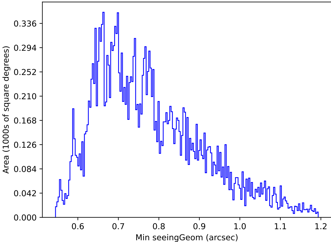
too_elab_r8_d2_ugrizy_v3.4_10yrs Yr 1 u band: Min seeingGeom
