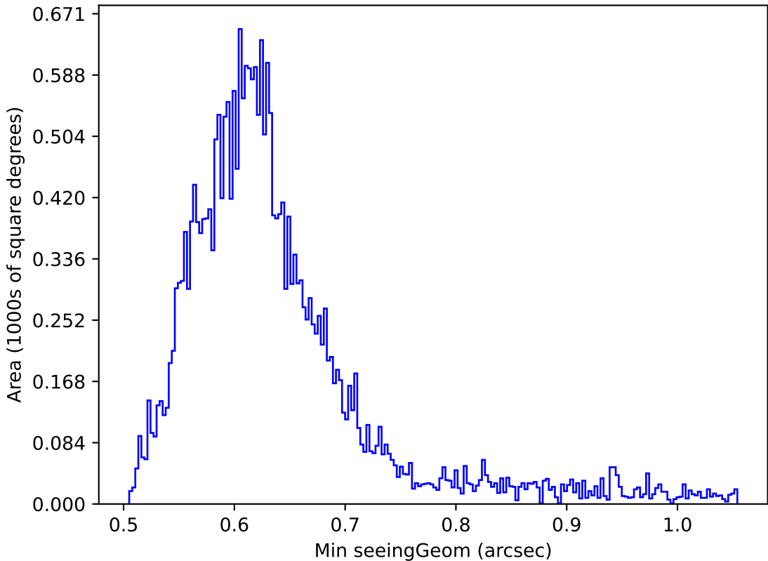
too_elab_r8_d2_ugrizy_v3.4_10yrs Yr 1 r band: Min seeingGeom
