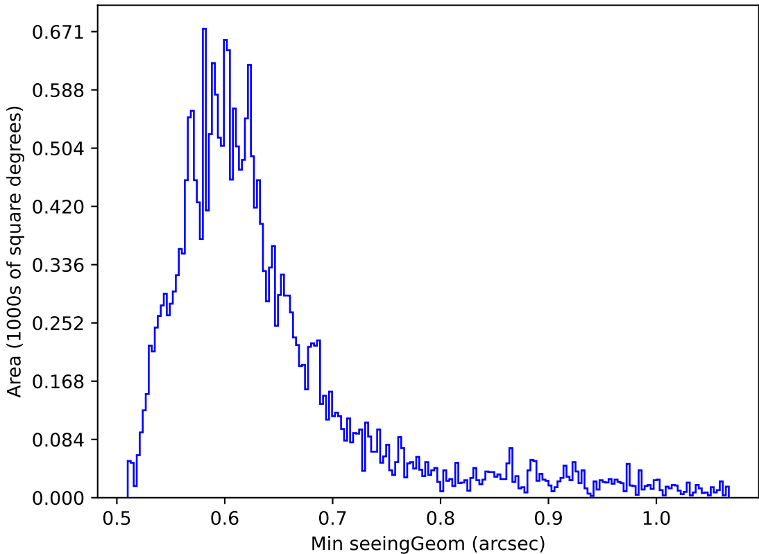
too_elab_r8_d2_ugrizy_v3.4_10yrs Yr 1 i band: Min seeingGeom
