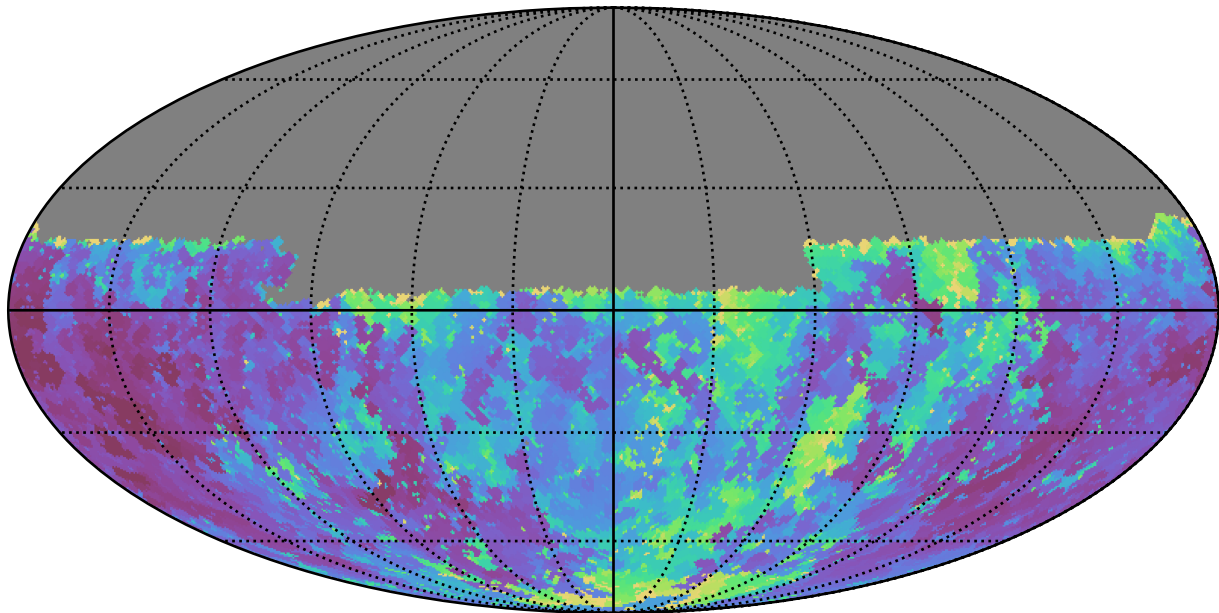
too_elab_r8_d2_ugrizy_v3.4_10yrs Yr 1 u band: Min seeingEff
