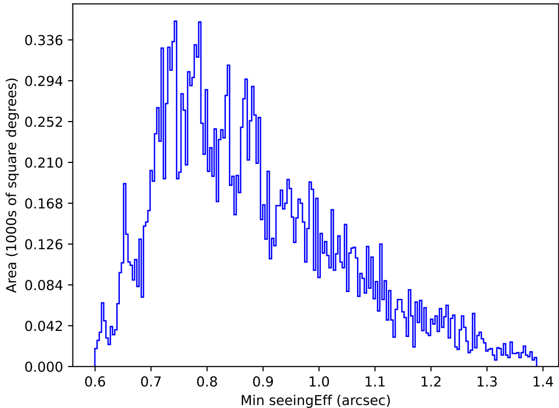
too_elab_r8_d2_ugrizy_v3.4_10yrs Yr 1 u band: Min seeingEff
