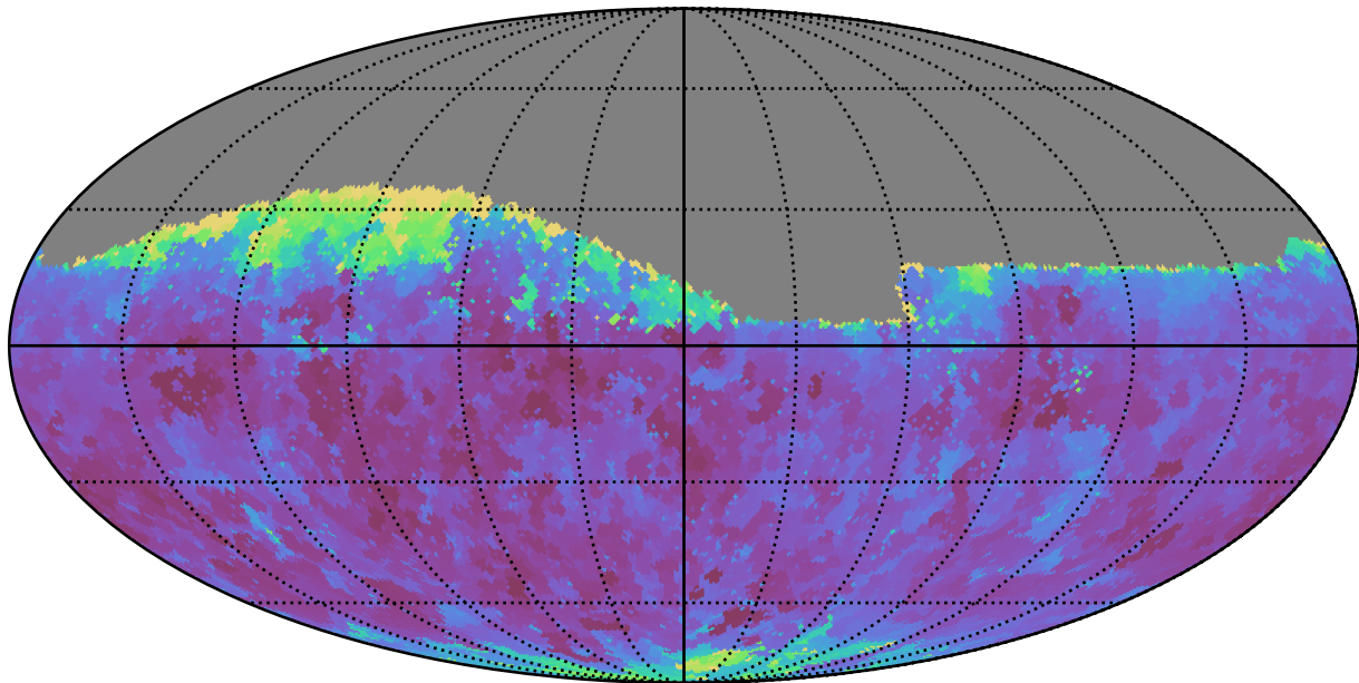
too_elab_r8_d2_ugrizy_v3.4_10yrs Yr 1 r band: Min seeingEff
