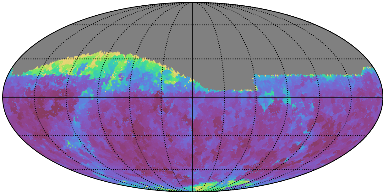
too_elab_r8_d2_ugrizy_v3.4_10yrs Yr 1 i band: Min seeingEff
