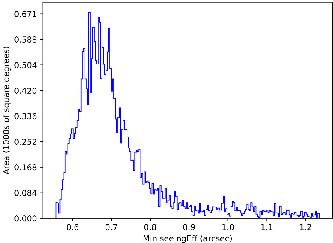
too_elab_r8_d2_ugrizy_v3.4_10yrs Yr 1 i band: Min seeingEff
