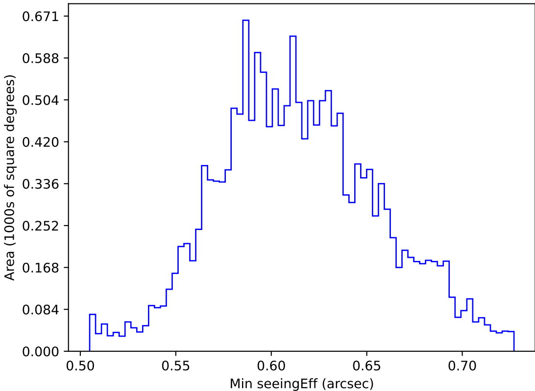
too_elab_r8_d2_ugrizy_v3.4_10yrs WFD z band: Min seeingEff
