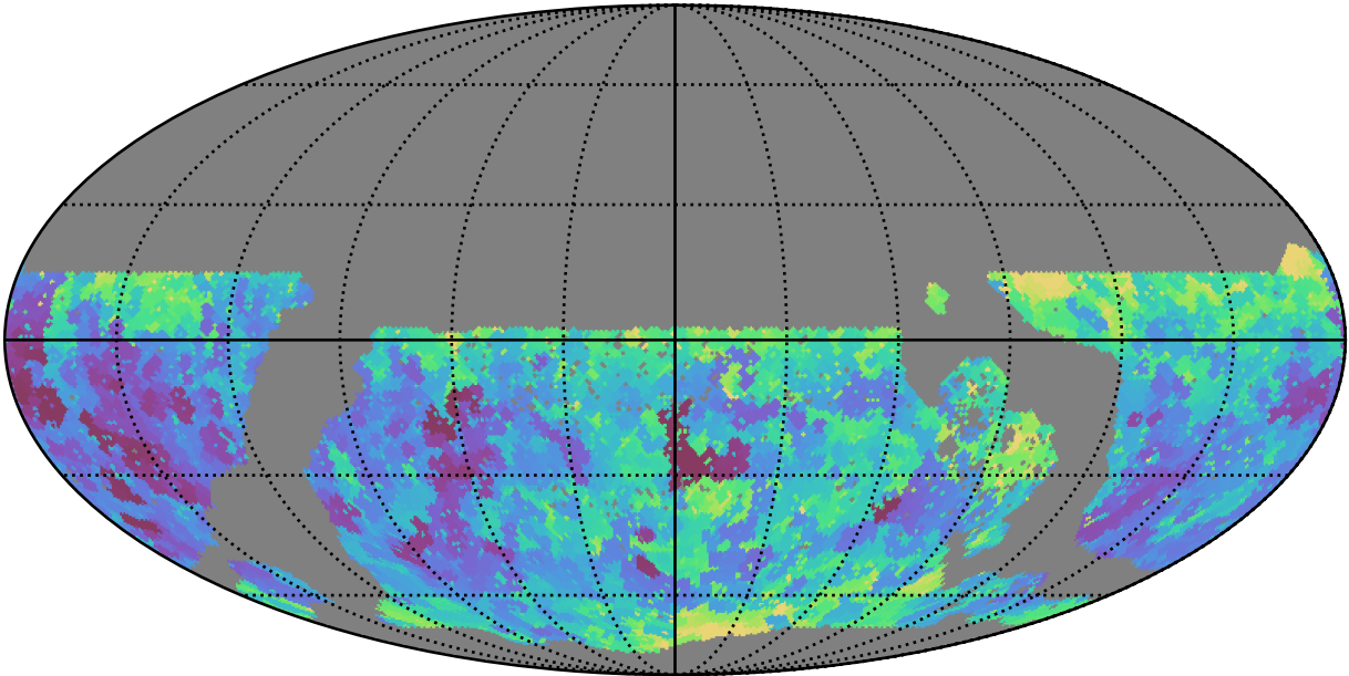
too_elab_r8_d2_ugrizy_v3.4_10yrs WFD u band: Min seeingEff
