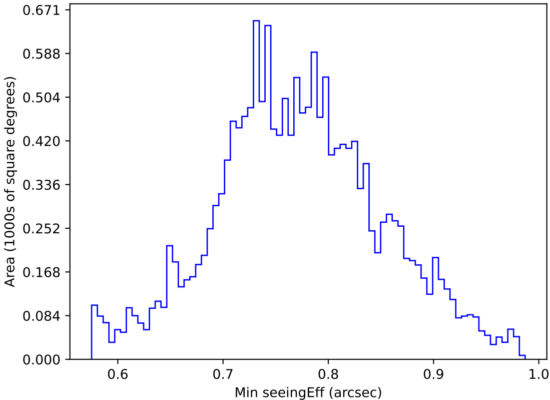
too_elab_r8_d2_ugrizy_v3.4_10yrs WFD u band: Min seeingEff
