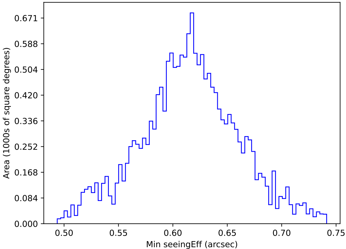
too_elab_r8_d2_ugrizy_v3.4_10yrs WFD r band: Min seeingEff
