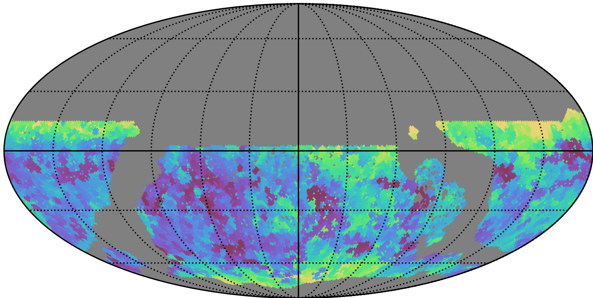
too_elab_r8_d2_ugrizy_v3.4_10yrs WFD i band: Min seeingEff
