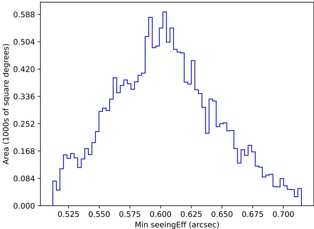
too_elab_r8_d2_ugrizy_v3.4_10yrs WFD i band: Min seeingEff
