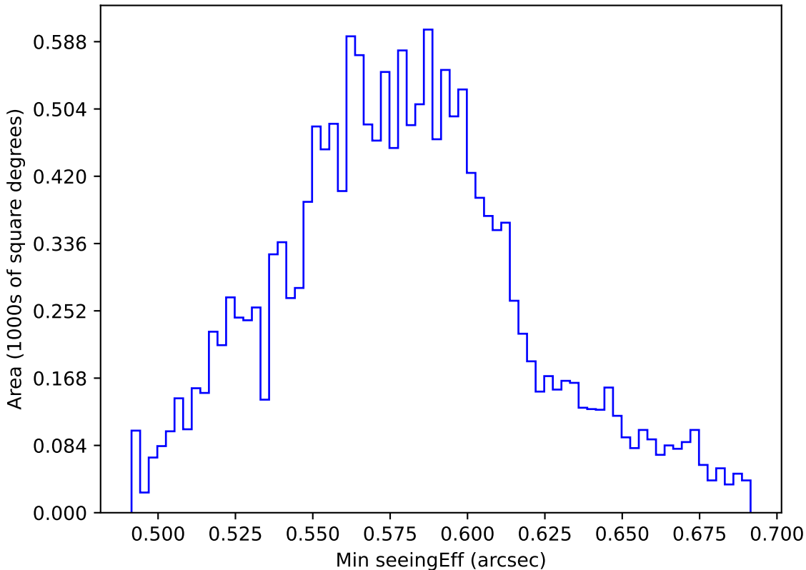
too_elab_r8_d2_ugrizy_v3.4_10yrs WFD all bands: Min seeingEff
