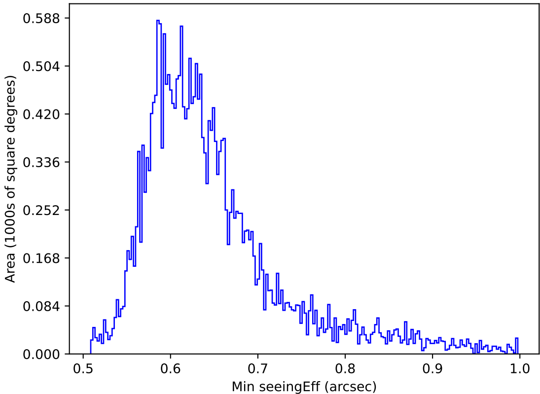
too_elab_r8_d2_ugrizy_v3.4_10yrs All sky z band: Min seeingEff
