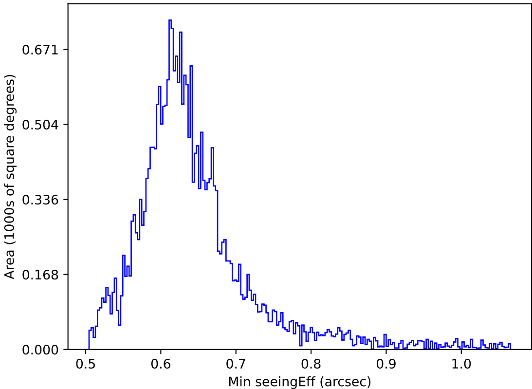
too_elab_r8_d2_ugrizy_v3.4_10yrs All sky r band: Min seeingEff
