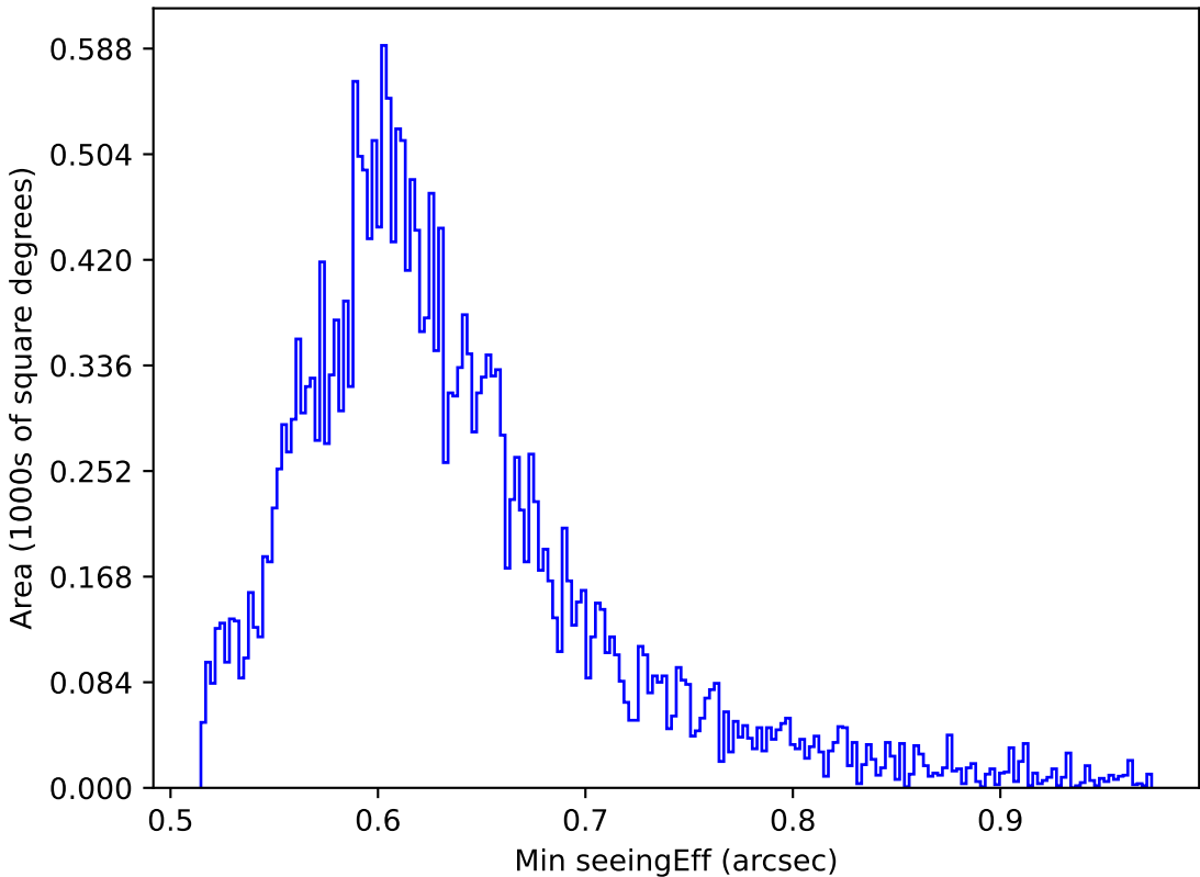
too_elab_r8_d2_ugrizy_v3.4_10yrs All sky i band: Min seeingEff
