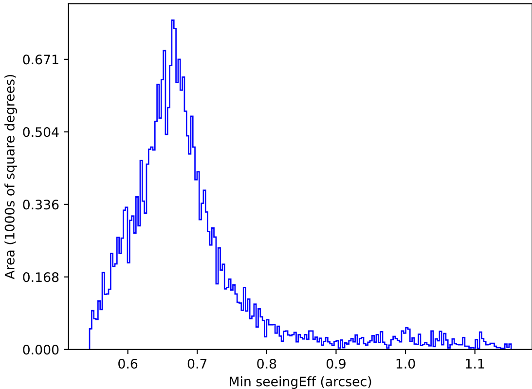
too_elab_r8_d2_ugrizy_v3.4_10yrs All sky g band: Min seeingEff
