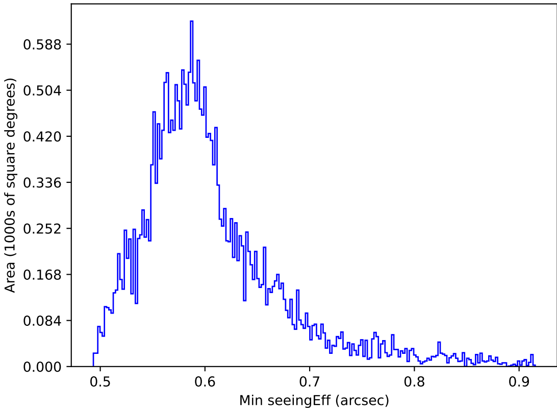
too_elab_r8_d2_ugrizy_v3.4_10yrs All sky all bands: Min seeingEff
