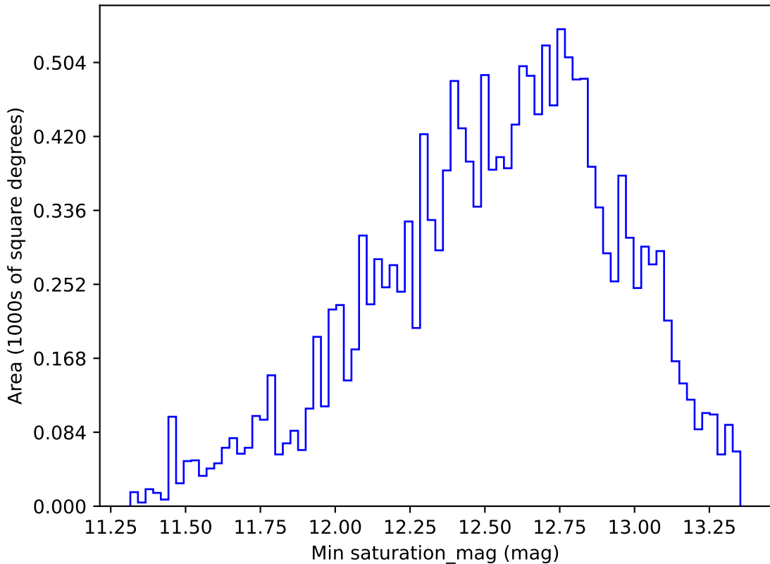
too_elab_r8_d2_ugrizy_v3.4_10yrs WFD r band: Min saturation_mag
