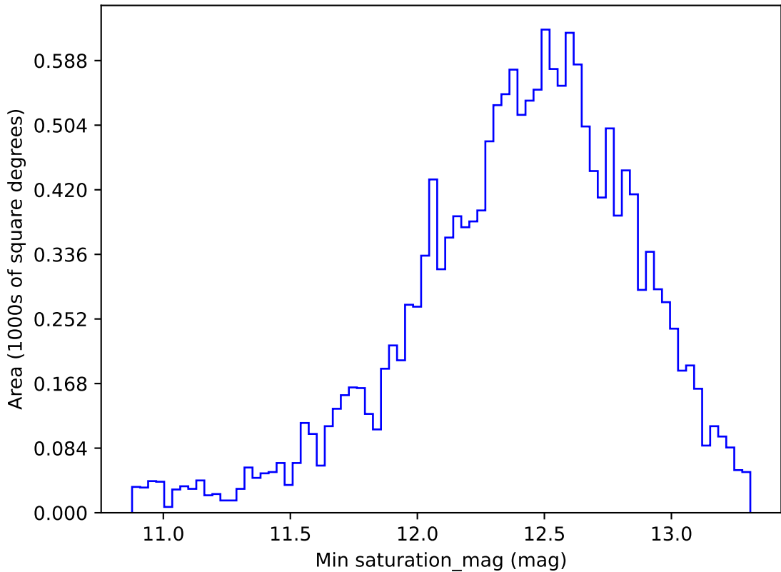
too_elab_r8_d2_ugrizy_v3.4_10yrs WFD i band: Min saturation_mag
