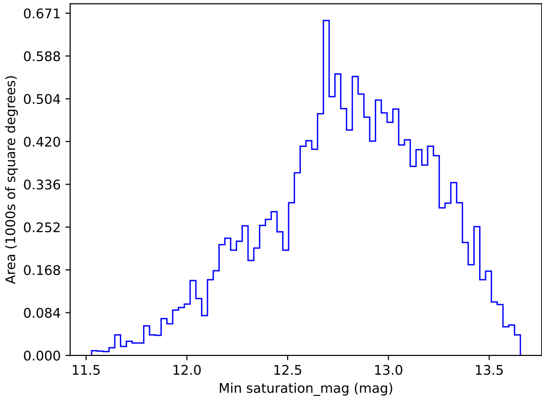
too_elab_r8_d2_ugrizy_v3.4_10yrs WFD g band: Min saturation_mag
