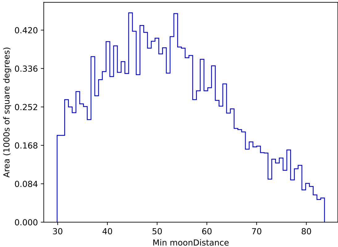
too_elab_r8_d2_ugrizy_v3.4_10yrs WFD u band: Min moonDistance
