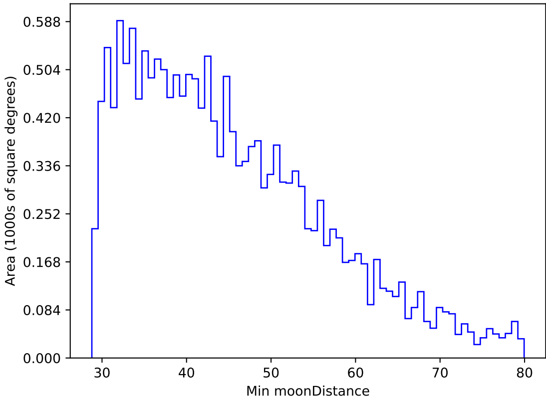
too_elab_r8_d2_ugrizy_v3.4_10yrs WFD g band: Min moonDistance
