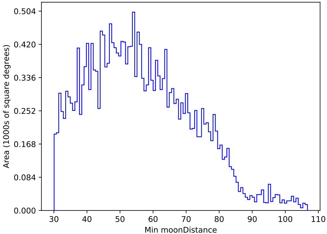
too_elab_r8_d2_ugrizy_v3.4_10yrs All sky u band: Min moonDistance
