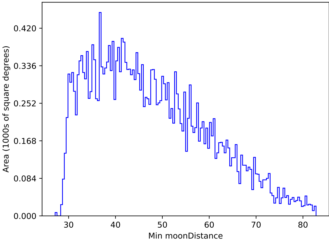
too_elab_r8_d2_ugrizy_v3.4_10yrs All sky g band: Min moonDistance
