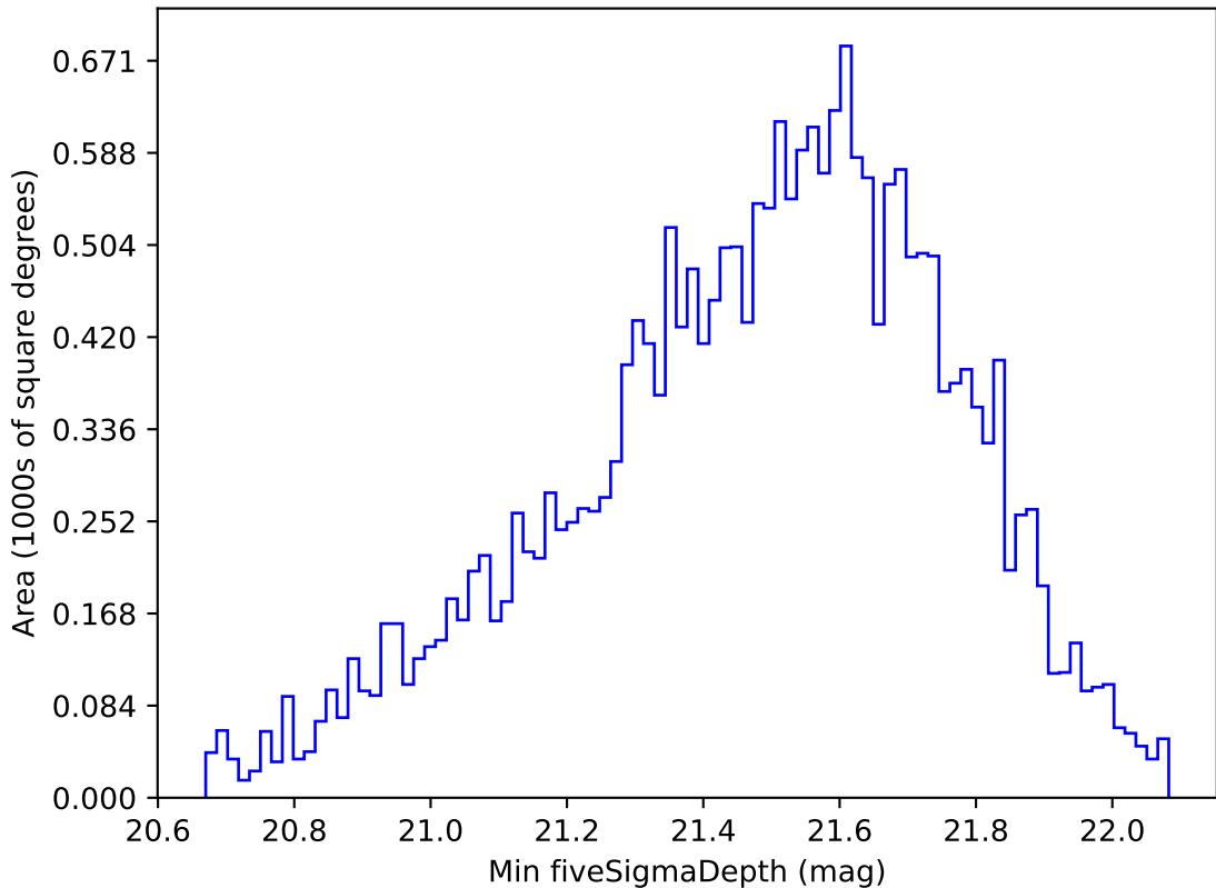
too_elab_r8_d2_ugrizy_v3.4_10yrs Yr 1 y band: Min fiveSigmaDepth
