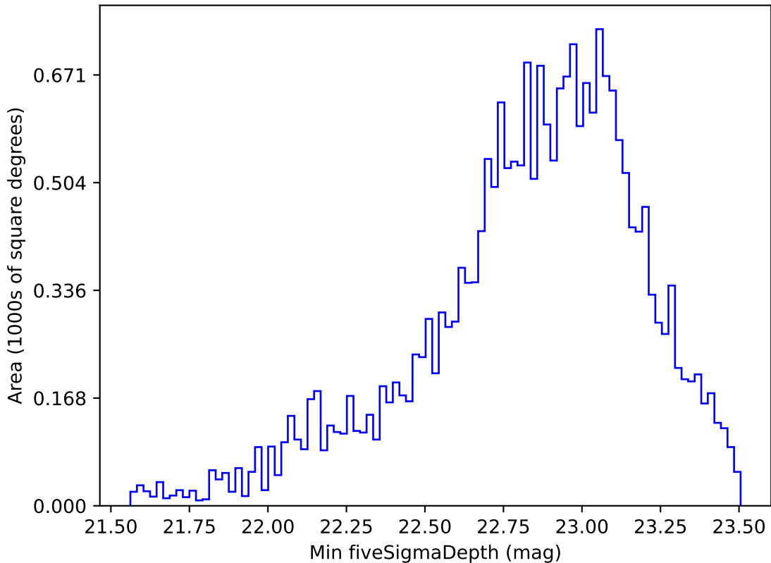
too_elab_r8_d2_ugrizy_v3.4_10yrs Yr 1 u band: Min fiveSigmaDepth
