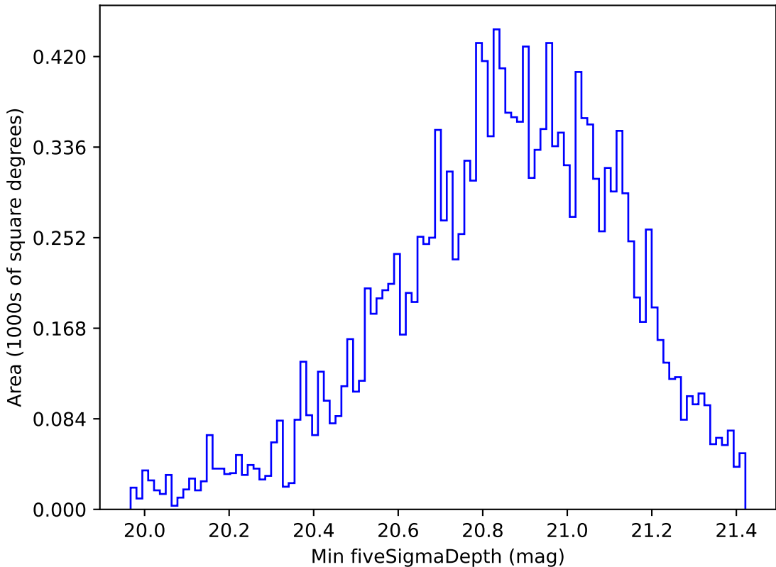
too_elab_r8_d2_ugrizy_v3.4_10yrs WFD y band: Min fiveSigmaDepth
