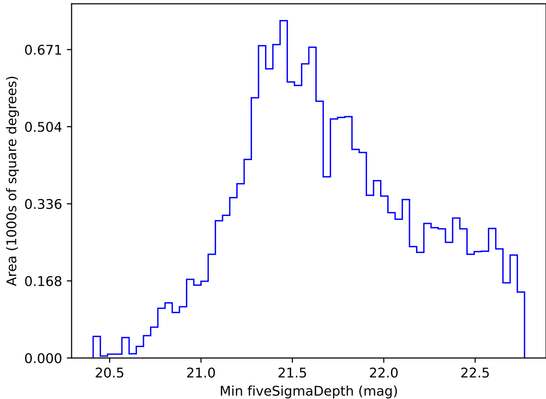
too_elab_r8_d2_ugrizy_v3.4_10yrs WFD i band: Min fiveSigmaDepth
