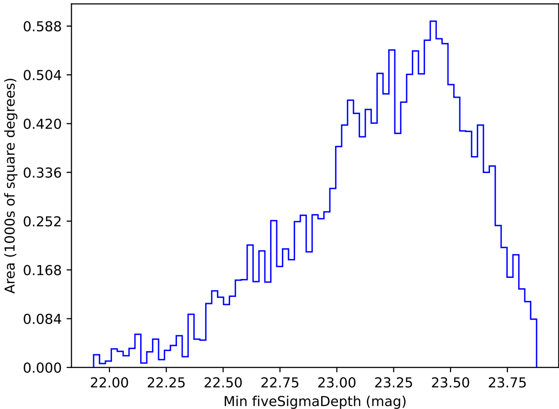
too_elab_r8_d2_ugrizy_v3.4_10yrs WFD g band: Min fiveSigmaDepth
