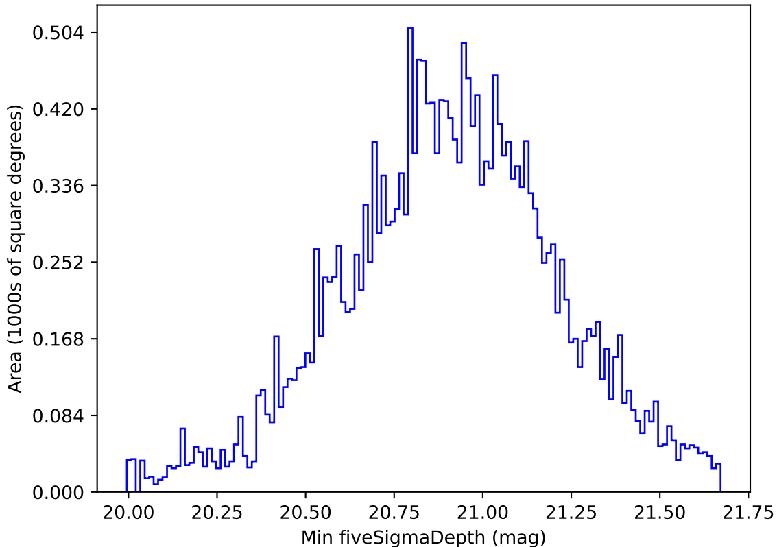
too_elab_r8_d2_ugrizy_v3.4_10yrs All sky y band: Min fiveSigmaDepth
