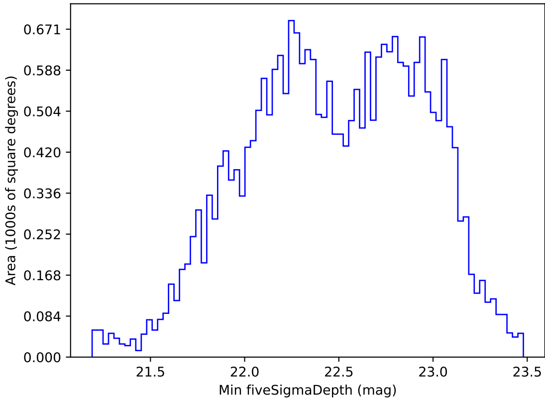
too_elab_r8_d2_ugrizy_v3.4_10yrs All sky r band: Min fiveSigmaDepth
