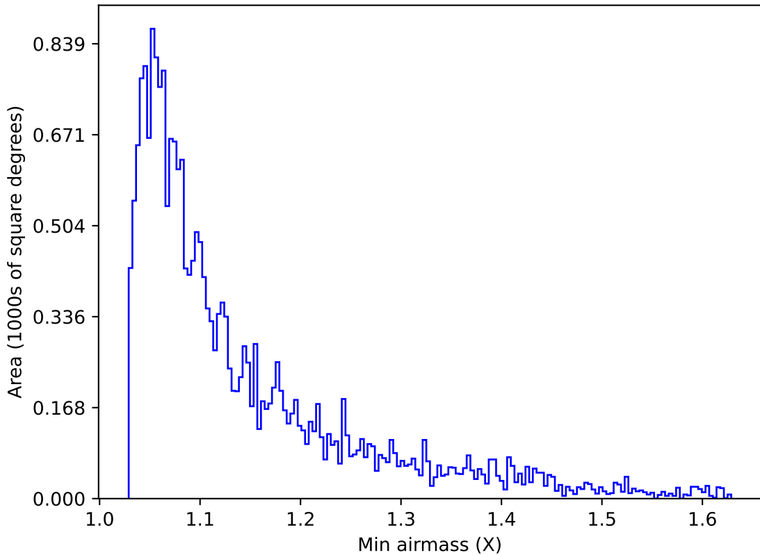
too_elab_r8_d2_ugrizy_v3.4_10yrs Yr 1 u band: Min airmass
