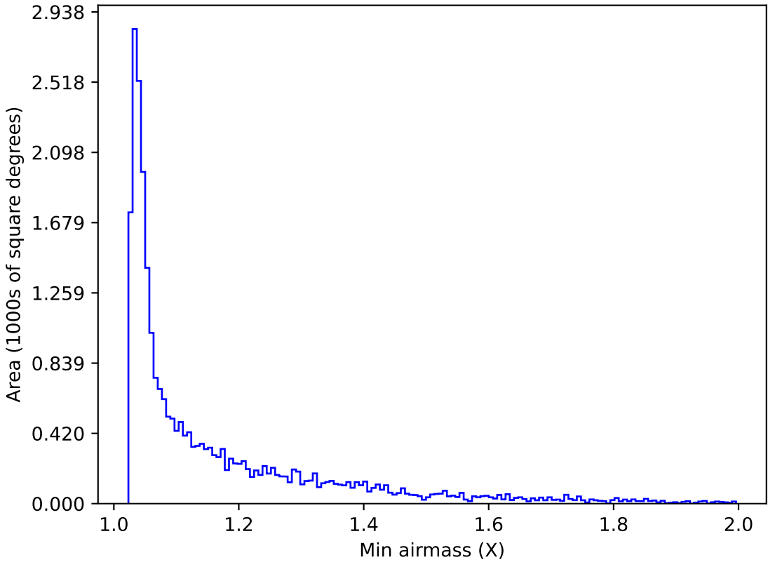
too_elab_r8_d2_ugrizy_v3.4_10yrs Yr 1 r band: Min airmass
