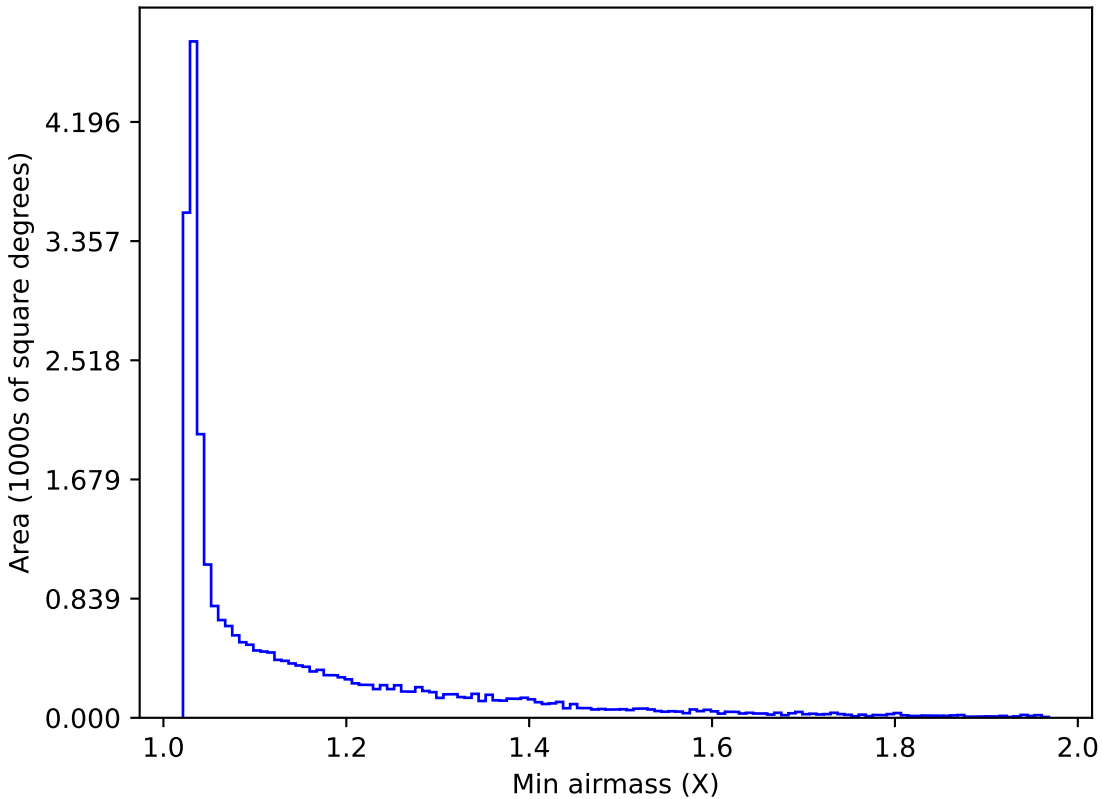
too_elab_r8_d2_ugrizy_v3.4_10yrs Yr 1 all bands: Min airmass
