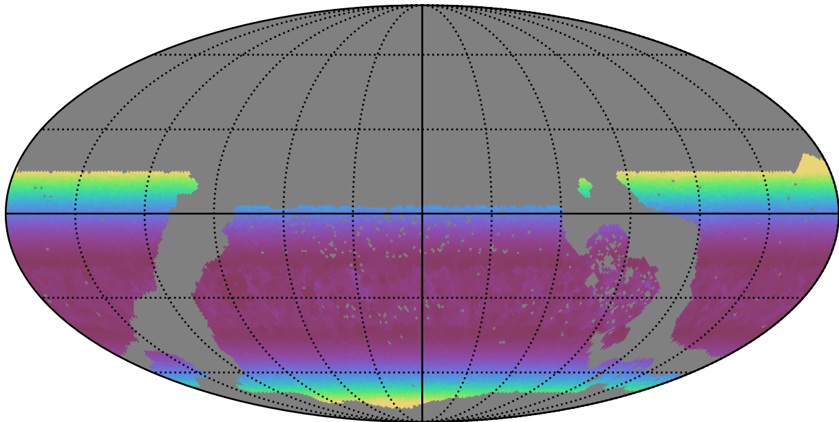
too_elab_r8_d2_ugrizy_v3.4_10yrs WFD u band: Min airmass
