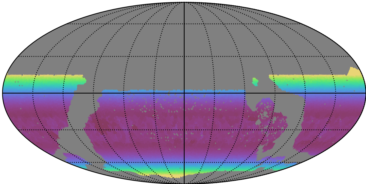
too_elab_r8_d2_ugrizy_v3.4_10yrs WFD g band: Min airmass
