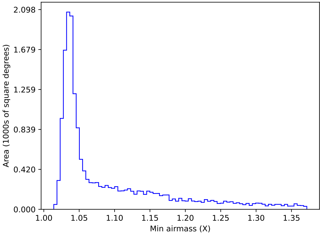
too_elab_r8_d2_ugrizy_v3.4_10yrs WFD g band: Min airmass
