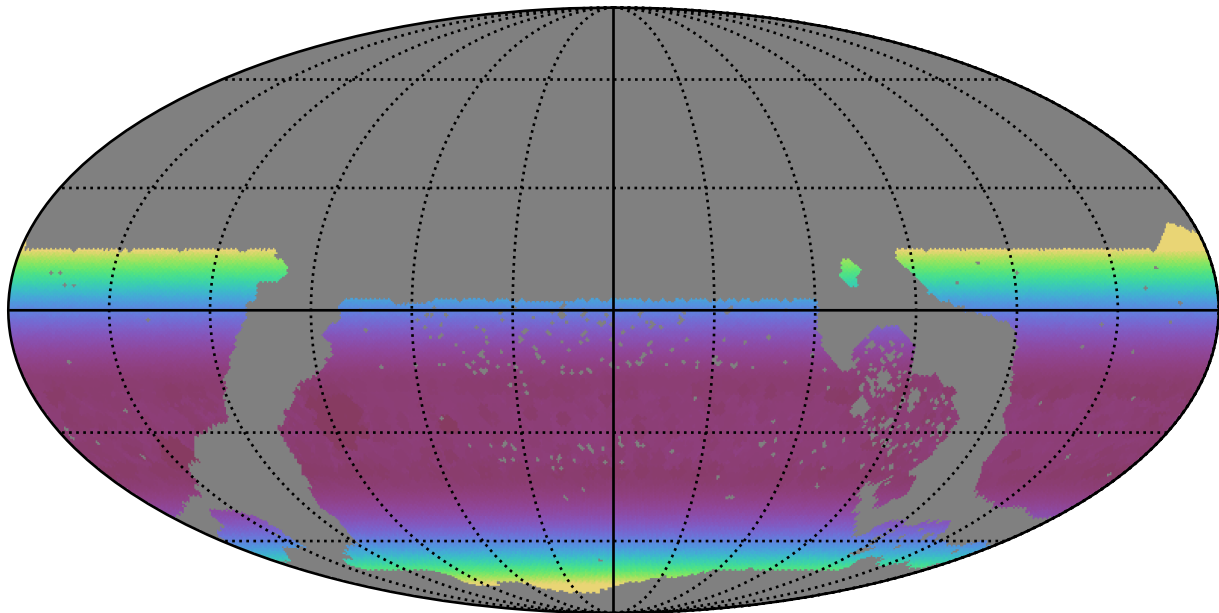
too_elab_r8_d2_ugrizy_v3.4_10yrs WFD all bands: Min airmass
