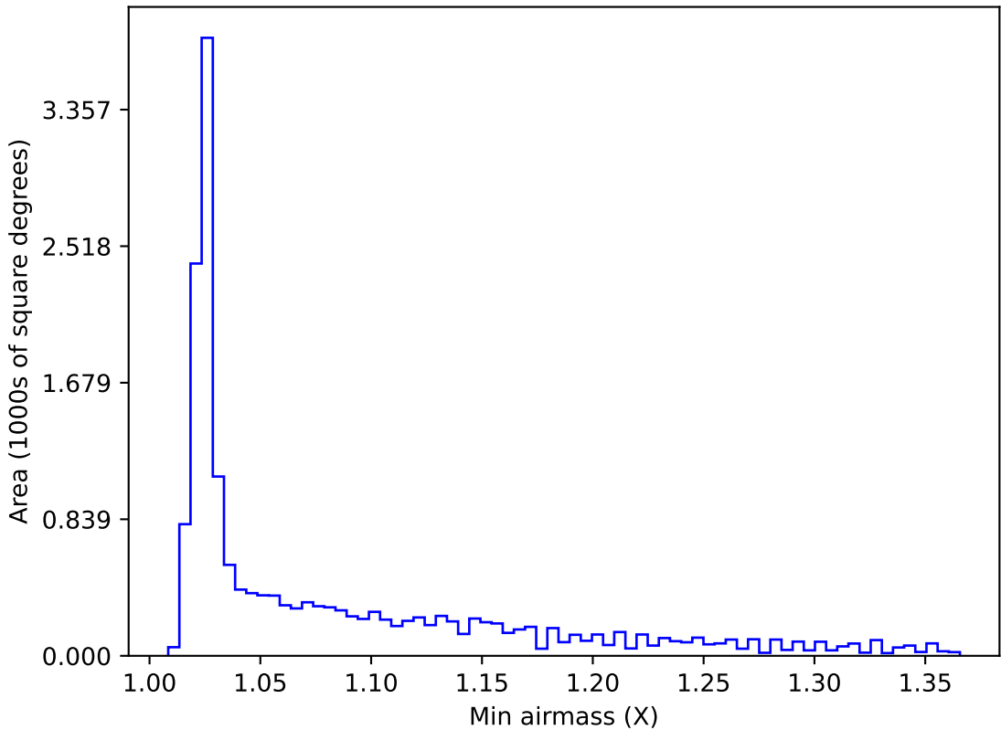
too_elab_r8_d2_ugrizy_v3.4_10yrs WFD all bands: Min airmass
