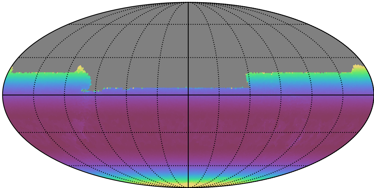
too_elab_r8_d2_ugrizy_v3.4_10yrs All sky y band: Min airmass
