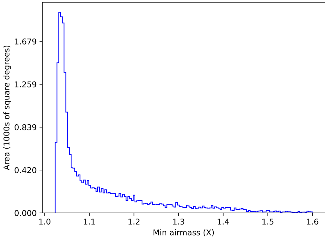
too_elab_r8_d2_ugrizy_v3.4_10yrs All sky u band: Min airmass
