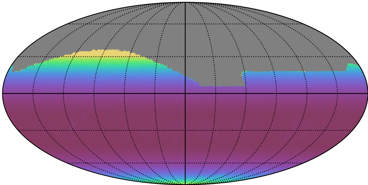
too_elab_r8_d2_ugrizy_v3.4_10yrs All sky r band: Min airmass
