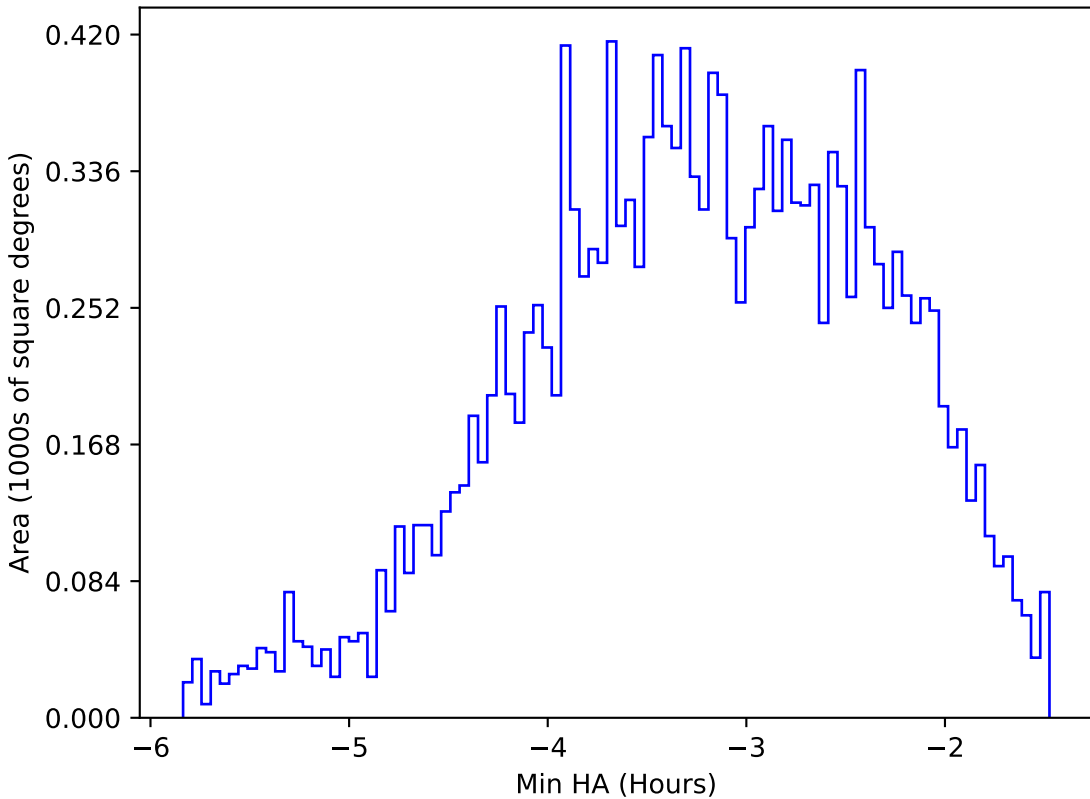
too_elab_r8_d2_ugrizy_v3.4_10yrs WFD u band: Min HA
